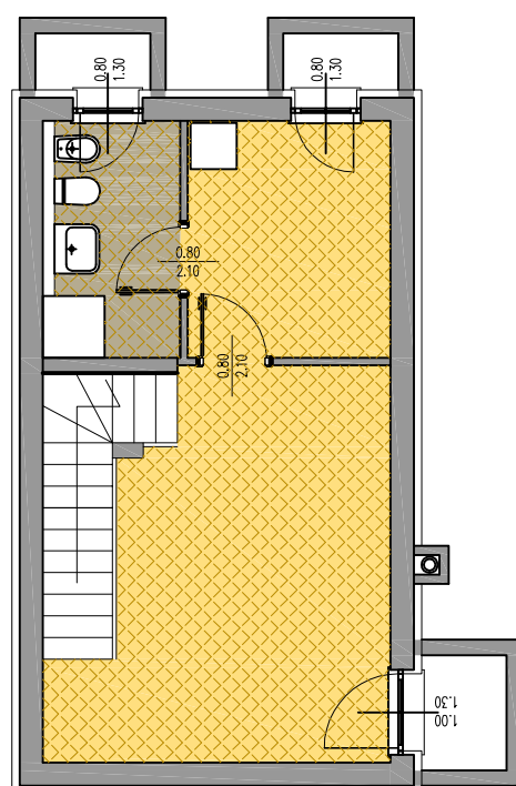
Piano Interrato
